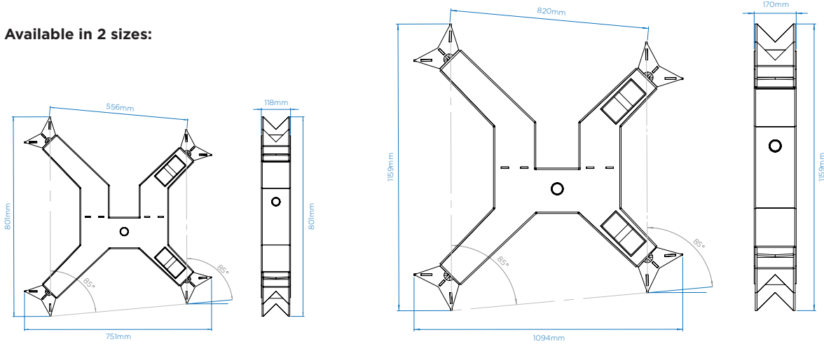
LW Stopper
